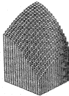
(c) m=n=16, V \approx 46.469
