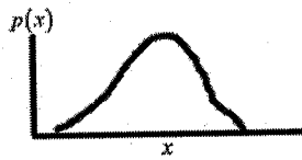
low negative skewness
