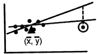
high leverage large residual, influential on slope
