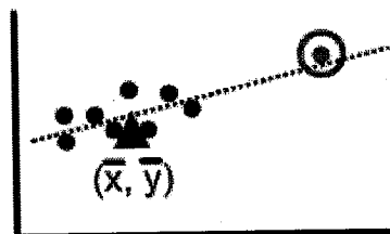
far from (\bar{x}, \bar{y}) in both x and y strongly affects correlation including this point strengthens correlation
