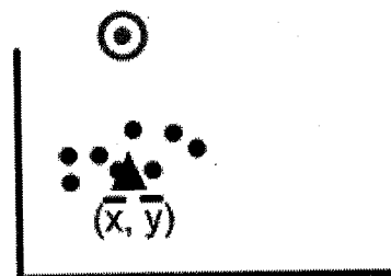
close to (\bar{x}, \bar{y}) in x little effect on correlation
