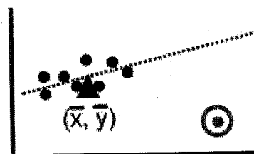
far from (\bar{x}, \bar{y}) in both x and y strongly affects correlation including this point weakens correlation
