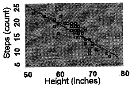
Scatterplot
