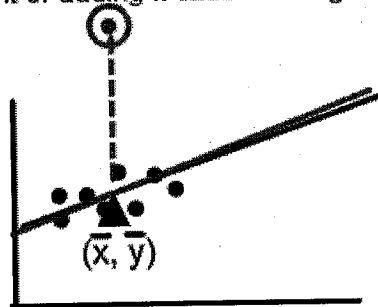
high residual but low leverage, not influential on slope
