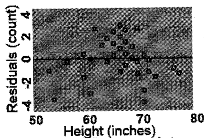
Linear model appropriate
