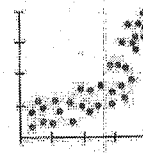
Non-Linear Association
