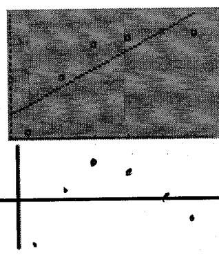
Residual plots
