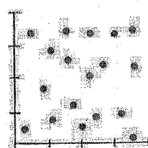
No Association
