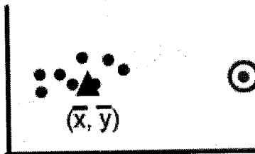
close to (\bar{x}, \bar{y}) in y little effect on correlation
