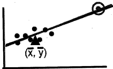
high leverage small residual, not influential on slope
