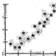
Positive Association (y increases as x increases)
